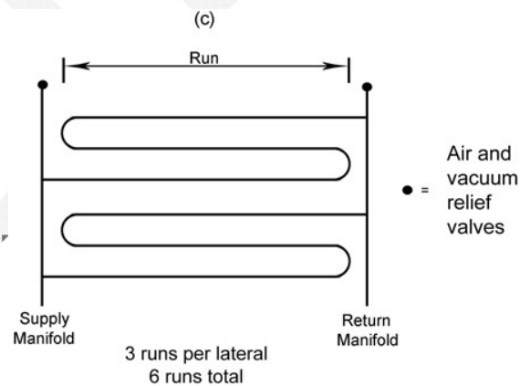
Illustrations of runs in various drip distribution configurations
