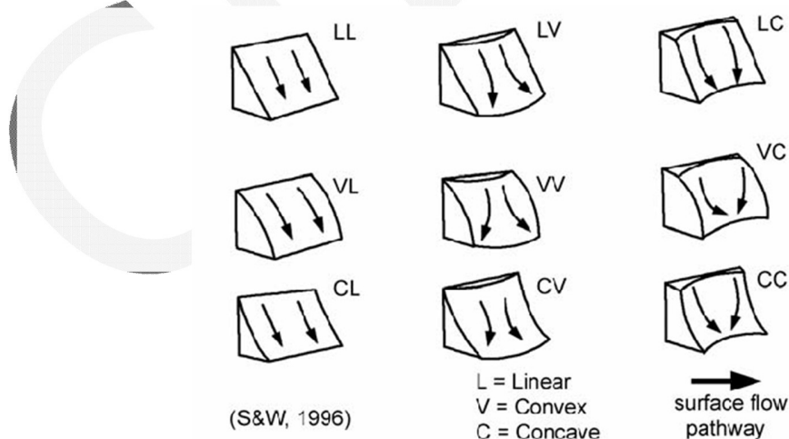
Slope shape descriptors
