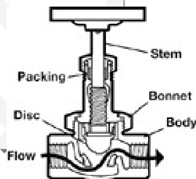
Globe valve
