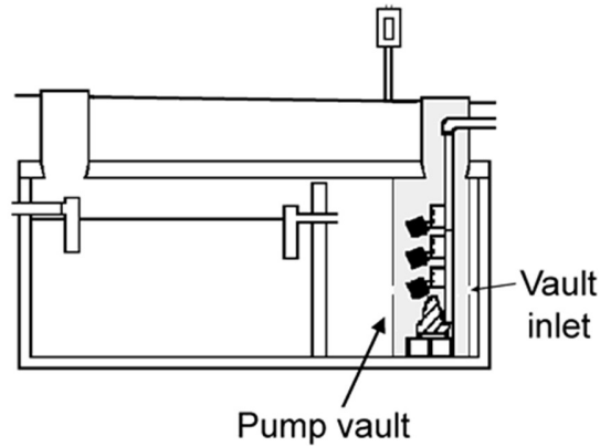
Pump installed within a pump vault
