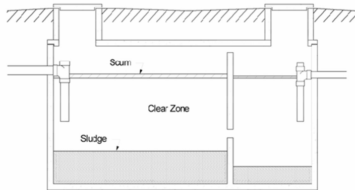
Clear zone of a two-compartment septic tank
