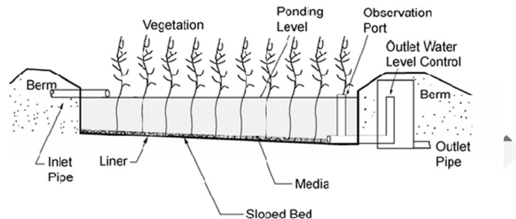
Free water surface constructed wetland system
