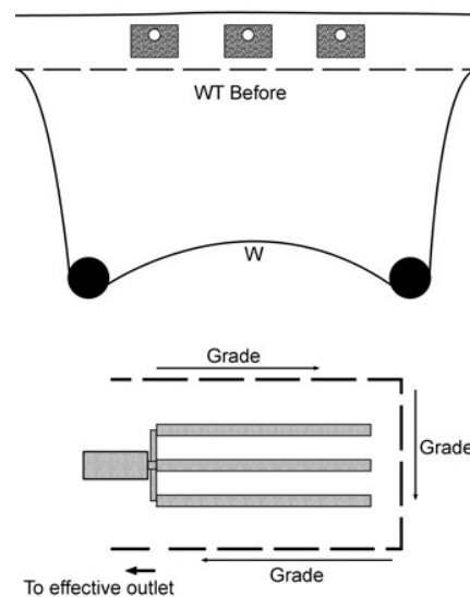
Perimeter drain ( section and plan view ) around a septic tank and soil treatment area
